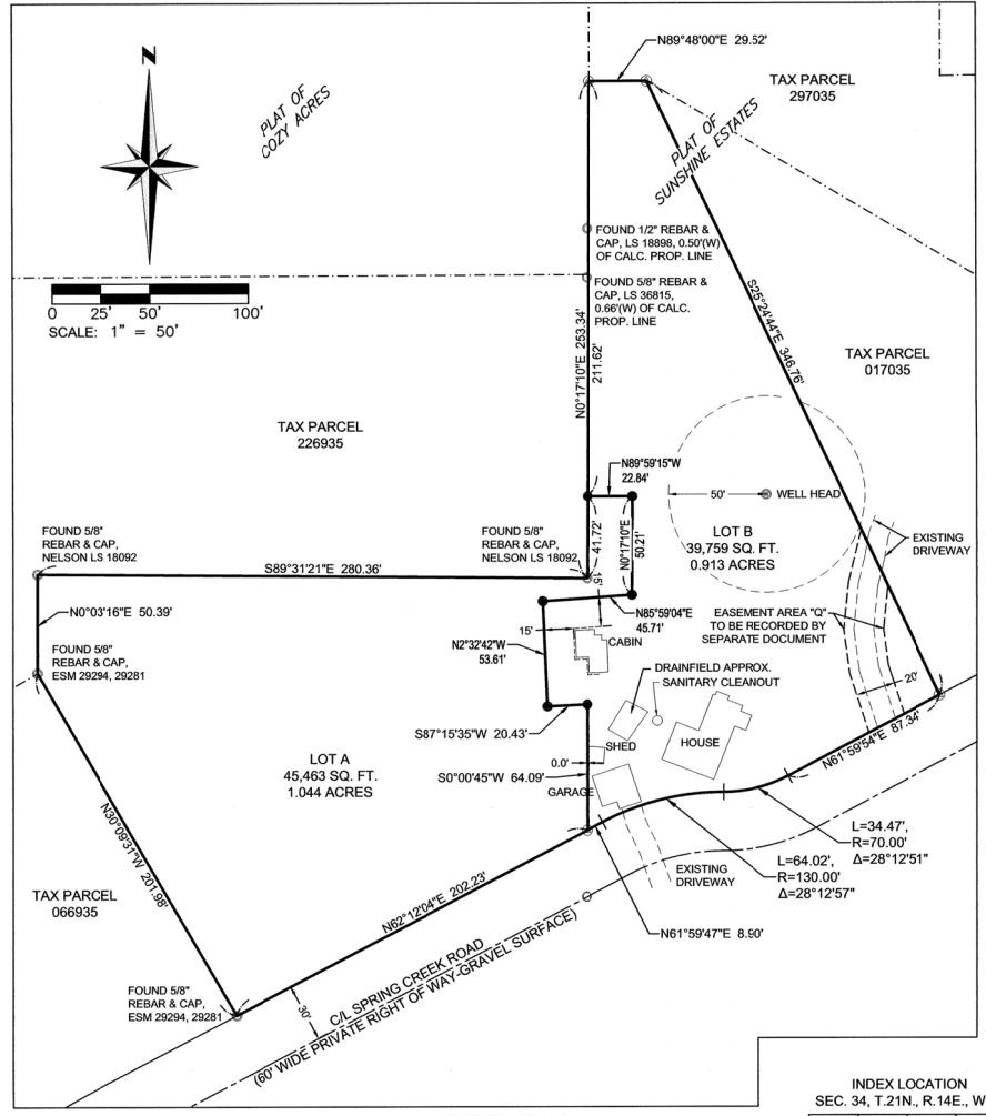
AFTER BLA
