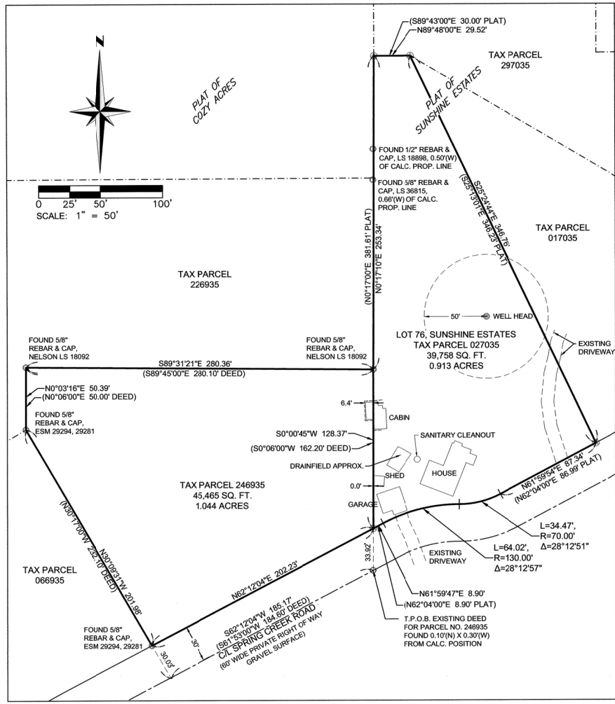
BEFORE BLA
